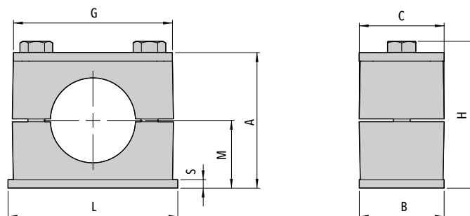
STANDARD SERIES (DIN 3015, Part 1) - mm (in)
