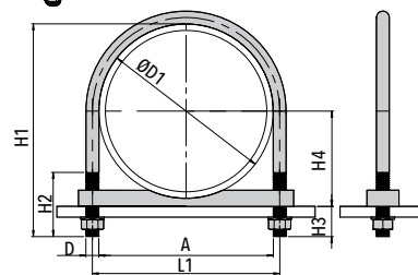
WITH LONG SADDLE BL
