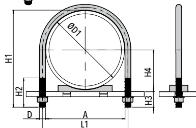
WITH SHORT SADDLE BC
